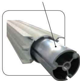
Aluminum tube \varnothing 52 mm to be anchor or resin fixed
