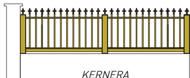
KERNERA with grooved bars Ø 23,5 mm Space between bars 102 mm
